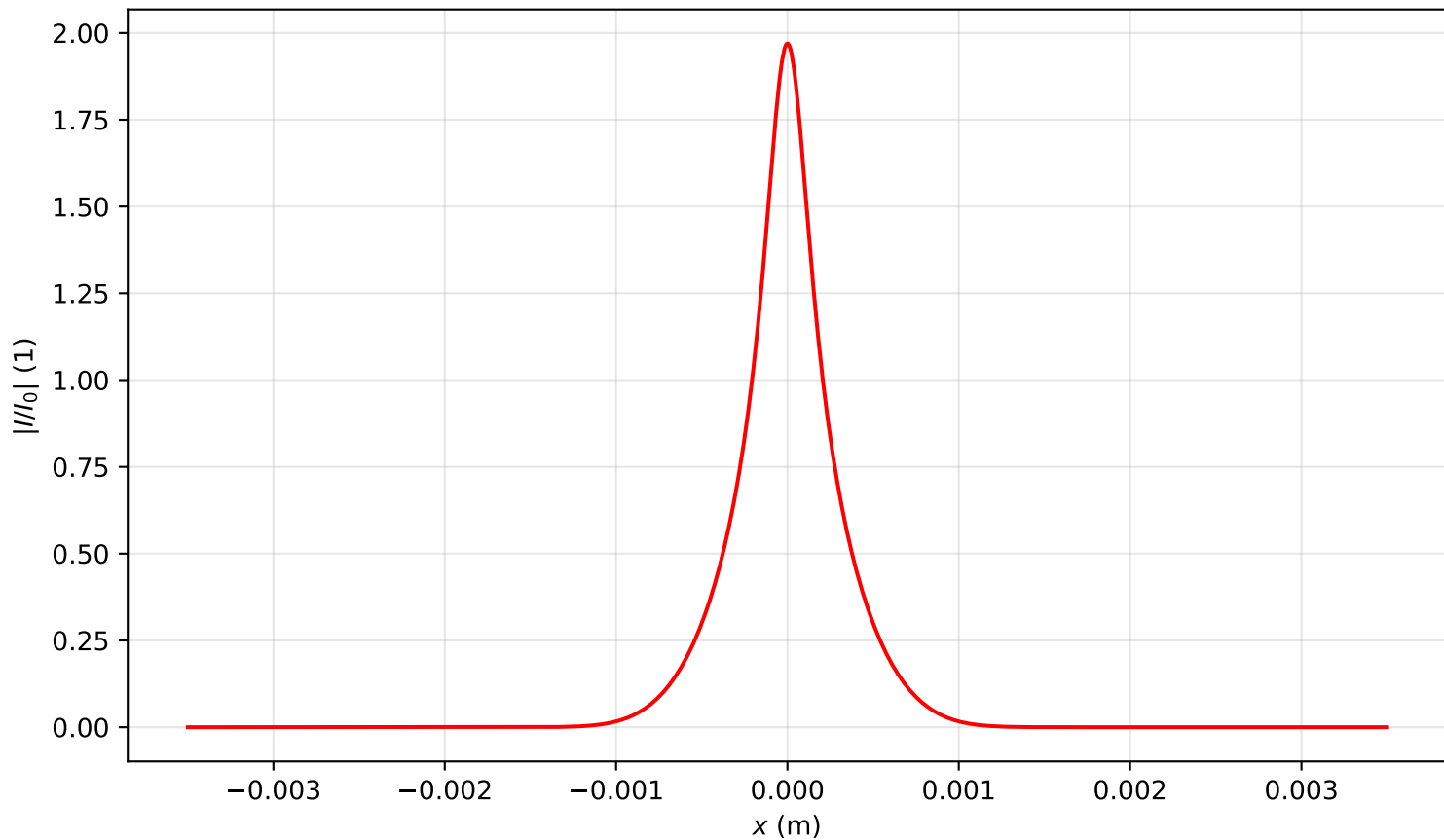
Intensity profile I(x, y = 0, z = 0.239)/I_0 , P_{in}=8.0P_{cr} , artificial time
